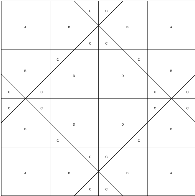
Worktable Block Pattern for 8.00x8.00 block Key Block (43/100 actual size)
